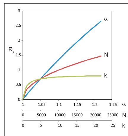
Figure 1. Relative impact of selectivity ( \alpha ), efficiency (N) and retention (k) on chromatographic resolution ( R_s ). Graphs were obtained by plotting the resolution equation [4] against one parameter while keeping the others fixed at the intersection point values ( \alpha=1.05 , N=5000 , k=5 ).
