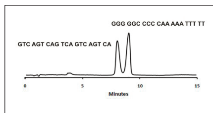
Figure 4. HILIC-MS separation of two 20 unit heterogeneous oligonucleotides of same composition but different sequence. Separation on ZIC-HILIC 100x2.1, 3.5 \mu m, 200 Å HPLC column at 50 °C, operated at 0.4 mL/min using linear gradient elution from 65% to 55% acetonitrile in water during 7.5 minutes with constant 10 mM ammonium acetate (pH 5.8). Courtesy of Lingzhi Gong, University of Oxford, UK [34].
