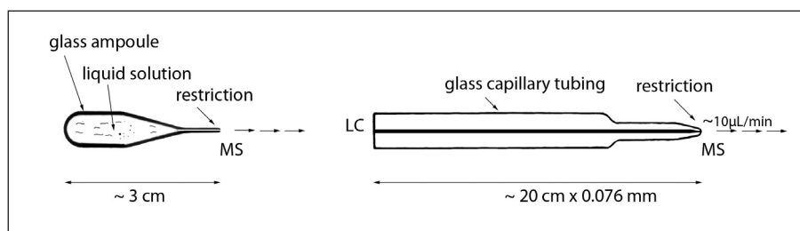
Figure 2: Left: schematic representation of the partly sealed ampoule used by M. Baldwin et al. [17] [18] to introduce liquid solutions directly within a MS ion source. Right: modified glass tube used by Arpino et al. [19] as a link between a HPLC system and a MS ion source.
