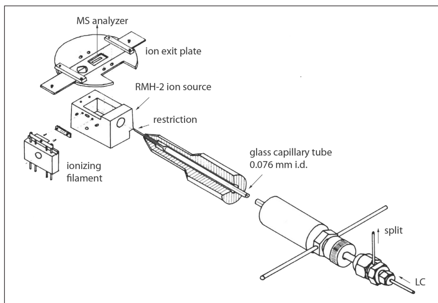
Figure 3: Inlet probe and MS source block for continuous introduction of solutions (adapted with permission from ref. 19)
